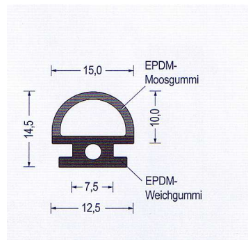
Art.-Nr. 2180001 EPDM 70°/20° schwarz VE : 100 m Bund
