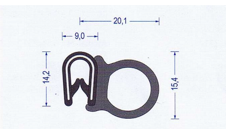
Art.-Nr. 2810011 · schwarz Klemmber.2-4 mm · VE: 50 m Bund Br* a50/b40/c100/d120
