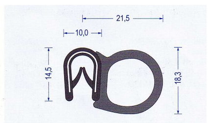
Art.-Nr. 2810012 · schwarz Klemmber.1-4 mm · VE: 50 m Bund Br* a50/b30/c100/d120
