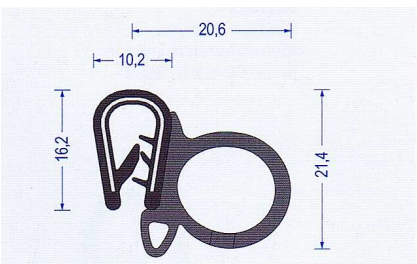
Art.-Nr. 2810007 · schwarz Klemmber.1-2,5 mm · VE: 50 m Bund Br* a60/b50/c120/d120
