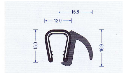
Art.-Nr. 2810003 · schwarz Klemmber.6-8 mm · VE: 50 m Bund Br* a60/b60/c170/d170
