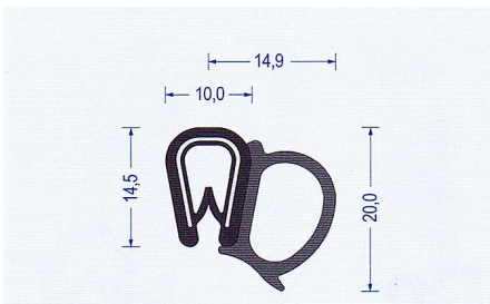
Art.-Nr. 2810005 · schwarz Klemmber.1-4 mm · VE: 50 m Bund Br* a60/b55/c80/d120
