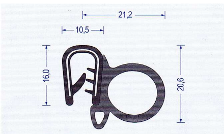
Art.-Nr. 2810008 · schwarz Klemmber.2,5-4 mm · VE: 50 m Bund Br* a60/b50/c120/d120
