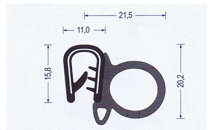
Art.-Nr. 2810009 · schwarz Klemmber.4-6 mm · VE: 50 m Bund Br* a60/b50/c120/d120
