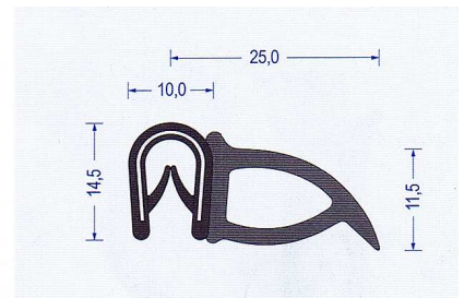
Art.-Nr. 2810006 · schwarz Klemmber.1-4 mm · VE: 50 m Bund Br* a50/b40/c140/d140
