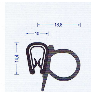
Art.-Nr. 2810020 schwarz Klemmbereich 1-4 mm VE: 50 m Bund Br* a100/b50/c80/d-
