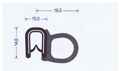
Art.-Nr. 2810010 · schwarz Klemmber.2-4 mm · VE: 50 m Bund Br* a50/b30/c100/d120
