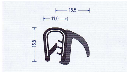
Art.-Nr. 2810002 · schwarz Klemmber.4-6 mm · VE: 50 m Bund Br* a60/b60/c160/d160
