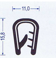
Art.-Nr. 2800019 schwarz Klemmber. 4 - 6 mm VE : 100 m Bund Br* a50/b40/c30/d30
