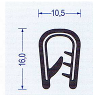
Art.-Nr. 2800018 schwarz Klemmber. 2 - 4 mm VE : 100 m Bund Br* a50/b40/c30/d30
