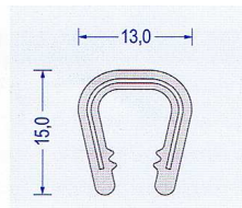
Art.-Nr. 2800022 hellgrau Klemmber. 6 - 8 mm VE : 100 m Bund Br* a40/b40/c40/d40
