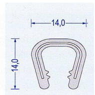
Art.-Nr. 2800024 hellgrau Klemmber. 8 - 10 mm VE : 100 m Bund Br* a40/b40/c40/d40
