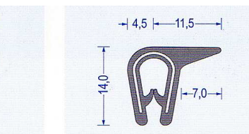
Art.-Nr. 2800027 anthrazit Klemmber. 1 - 3 mm VE : 100 m Bund Br* a125/b25/c80/d75
