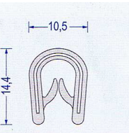
Art.-Nr. 2800013 hellgrau Klemmber. 1 - 4 mm VE : 100 m Bund Br* a30/b20/c20/d20
